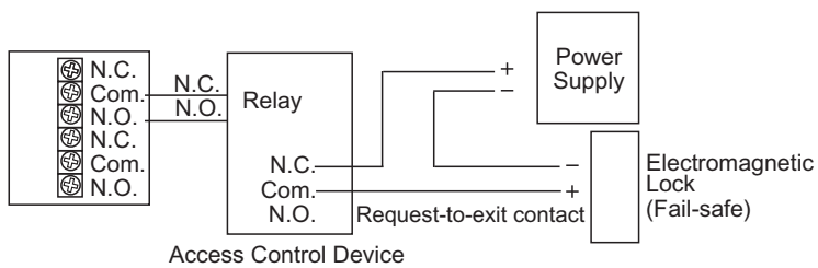
Connect the access control device
