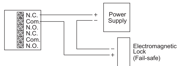
Directly control the fail-safe electromagnetic lock
