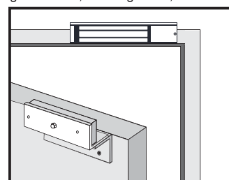
LZ-bracket for inswing doors
