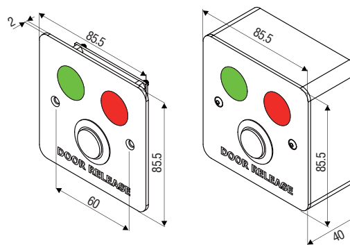
TLM-250
